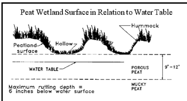
Figure TH-10: The water table (solid line) is near the bottom of the hollows (upper dotted line). Operations should stop when ruts reach 6 inches below the water table or 6 inches below the bottom of the hollows, whichever is lower. Peat is usually still porous 9 inches below the hollows, and ruts will heal in 2 to 3 years. Deep ruts (more than 12 inches below the hollows) will bring up well-decomposed, mucky peat and may take more than 20 years to heal.
