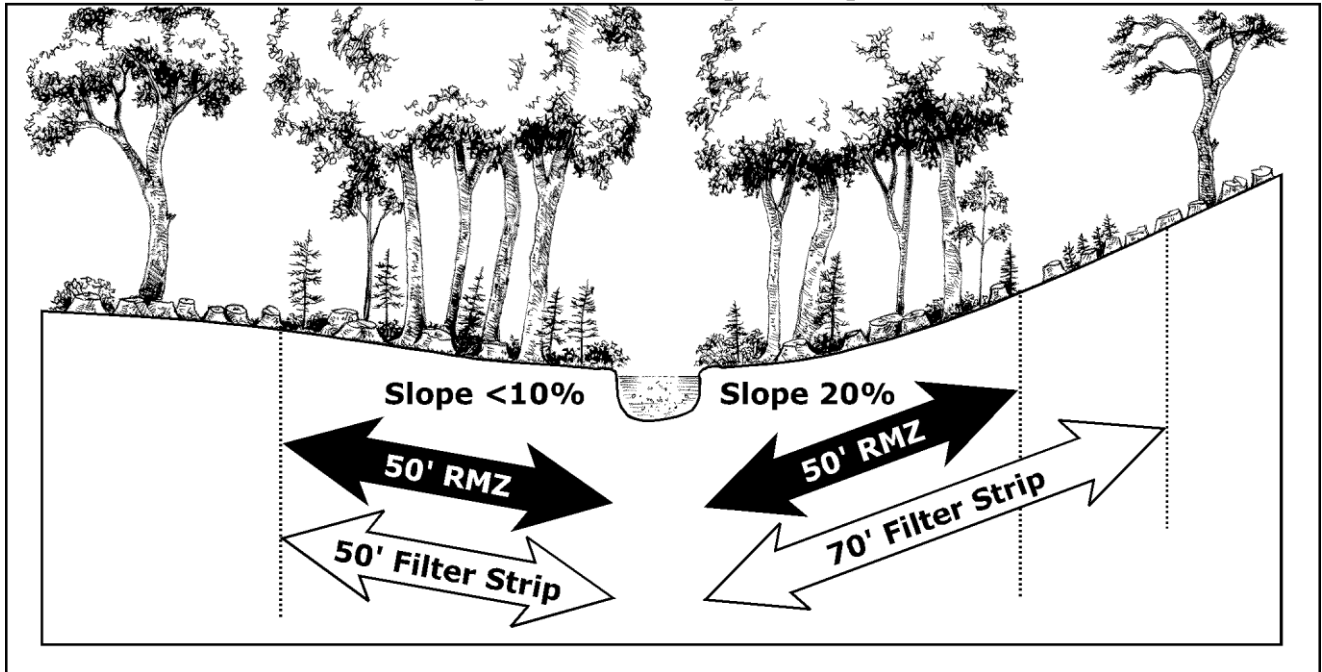
Figure GG-4 Filter Strips and RMZ for Non-Trout Perennial Streams < 3 Feet Wide of Varying Slopes
