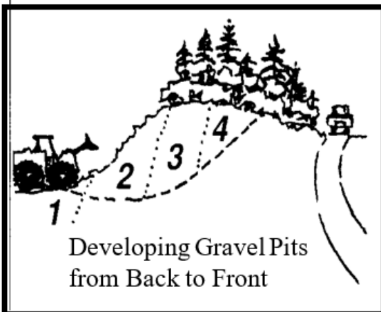
Figure ROAD-6: Develop gravel pits from back to front, moving toward predominant viewer or vantage point. In this illustration, Stage 1 has been completed, Stage 2 is in process, and Stages 3 and 4 will follow. Leaving the area adjacent to the road beyond Stage 4 untouched could result in no negative visual impact on the travel route.
