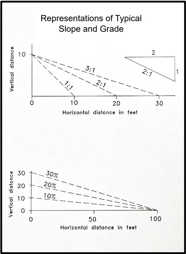
Figure ROAD-4. Representations of typical slope and grade.
