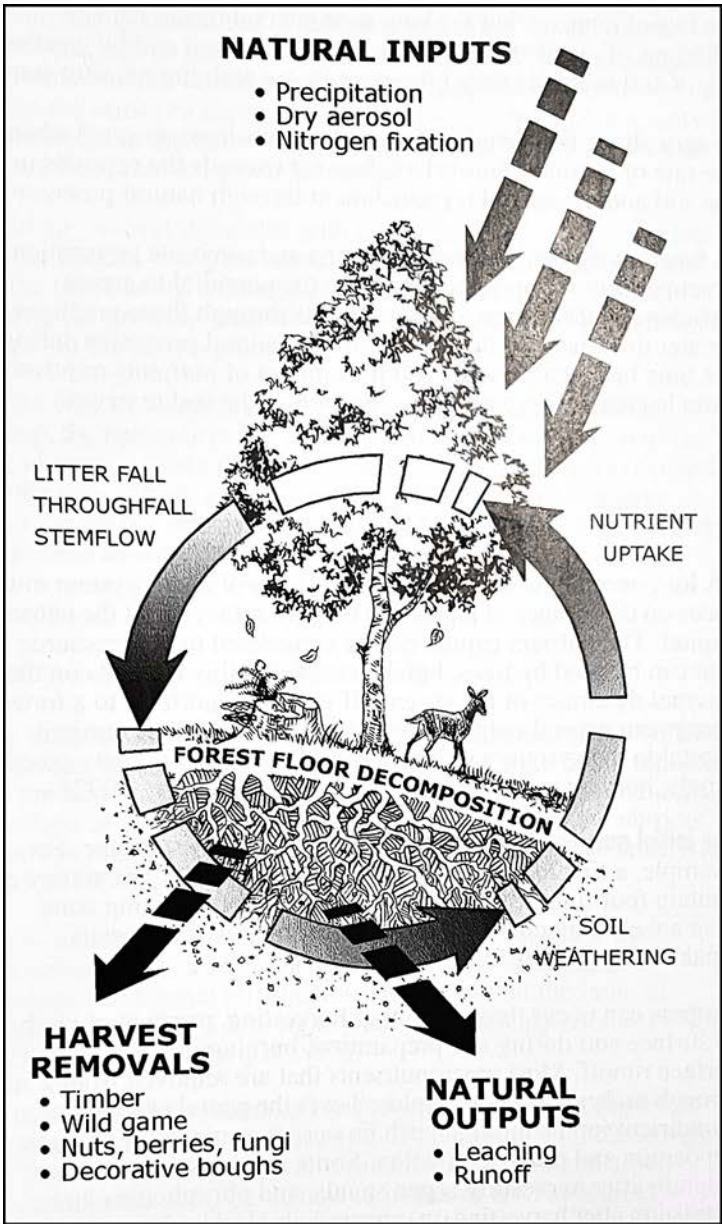
Figure S-2 Nutrient Cycling
