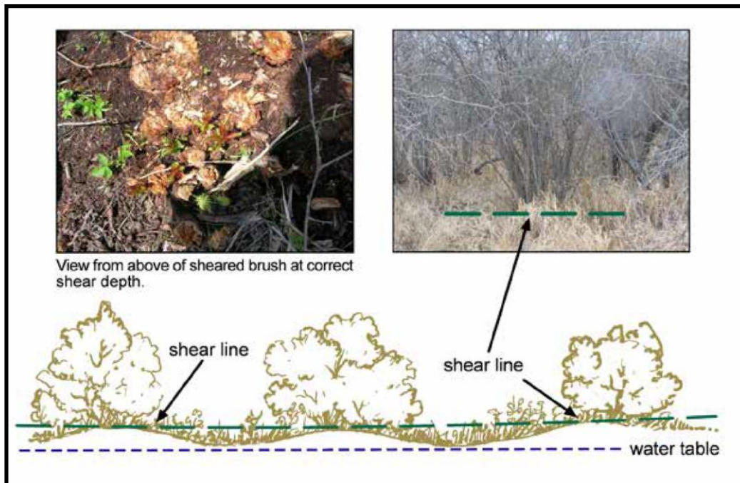
Figure BHB-4 - Shearing Hummocks
