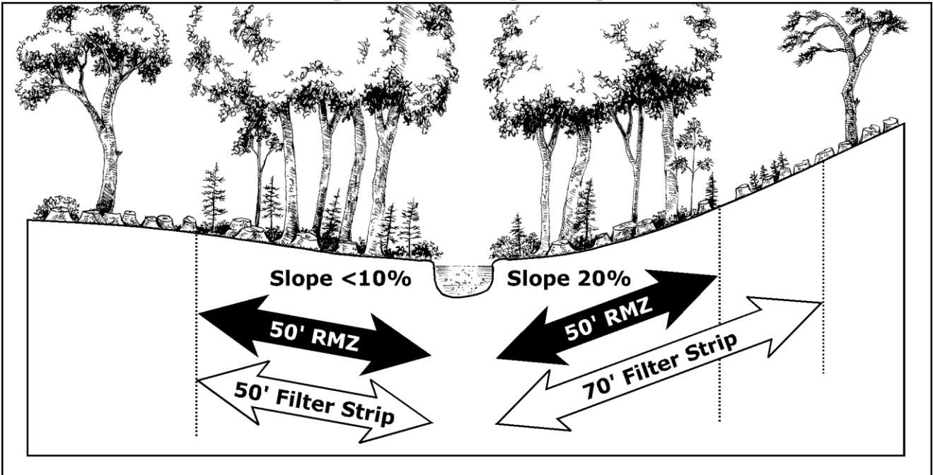
Figure GG-4 Filter Strips and RMZ for Non-Trout Perennial Streams < 3 Feet Wide of Varying Slopes
