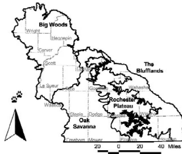
Figure 1. Ecological subsections in the Southeast landscape.
