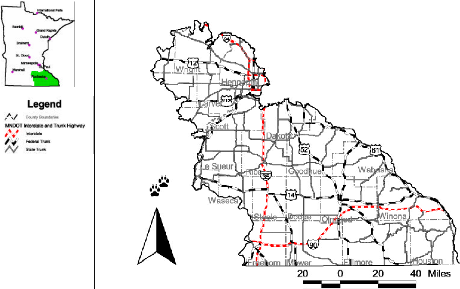
Figure 19. Major roads in the Southeast ecological landscape.
