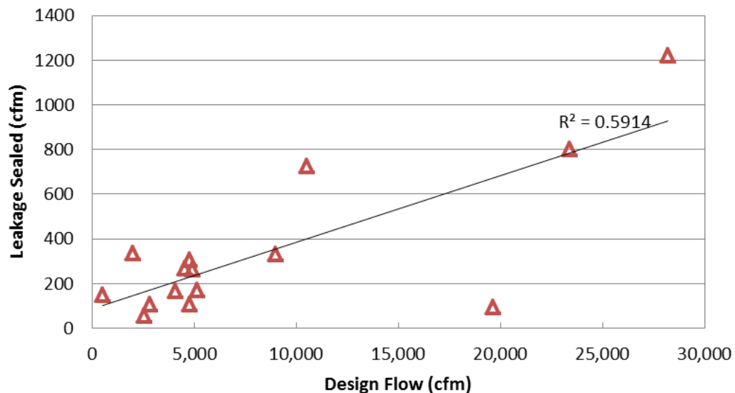
Figure 32: Sealed leakage as a function of design flow for successful sealing projects (n = 15)
