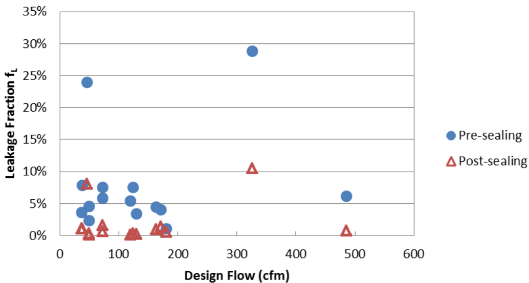
Figure 31: Pre and post leakage fractions for successful sealing projects (n = 15)
