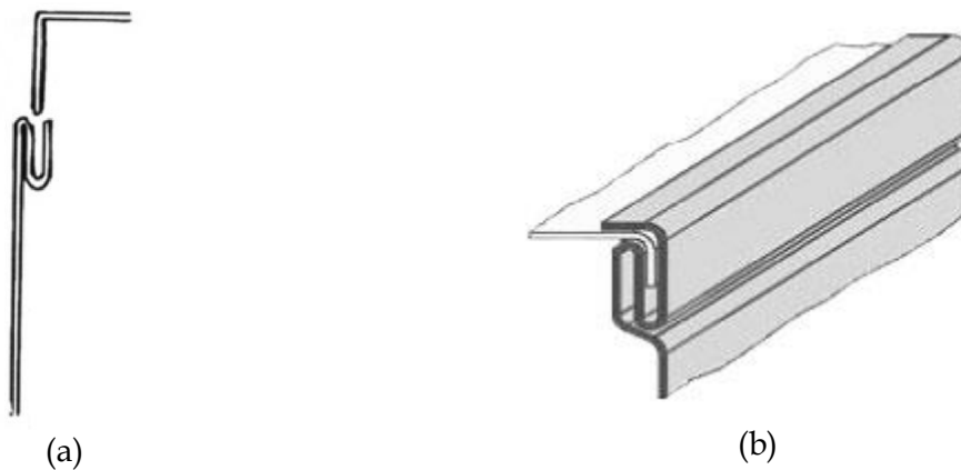
Figure 7: Examples of longitudinal seams found in sheet metal ductwork (a) tongue and groove 1 and (b) Pittsburgh Lock 2
