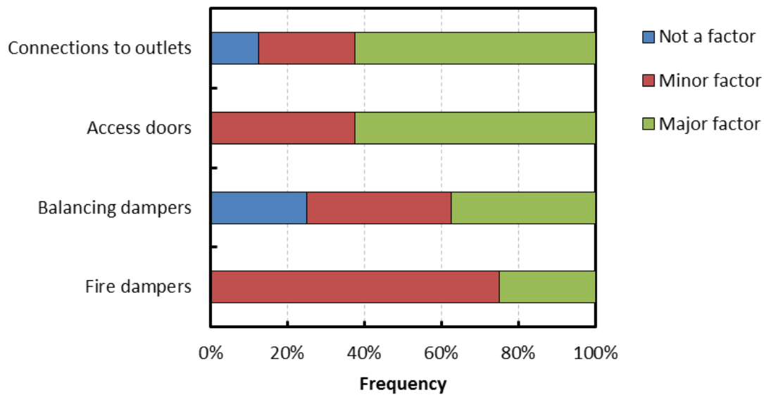
Figure 16: Contribution of accessories to leakage (n = 8)
