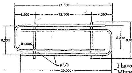
UPPER ARMASON REINFORCEMENT SCALE 1/8
