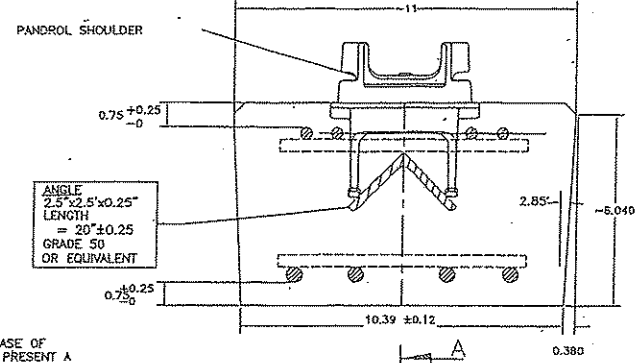
PARTIAL VIEW OF SUPPORT BASE SCALE 1/8
