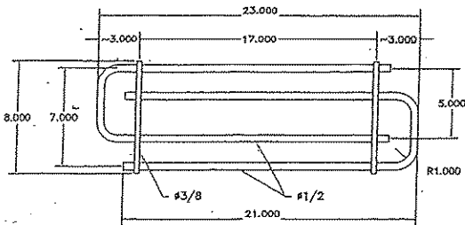
LOWER ARMASON REINFORCEMENT SCALE 1/8
