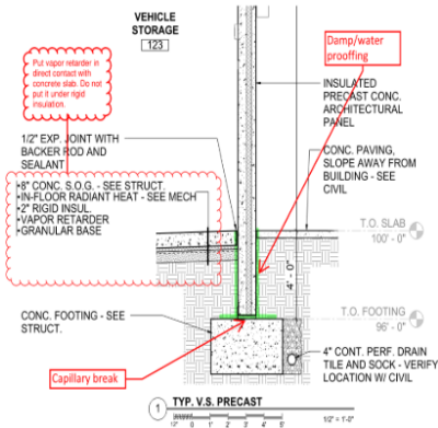
Capillary control at wall to footing details needed
