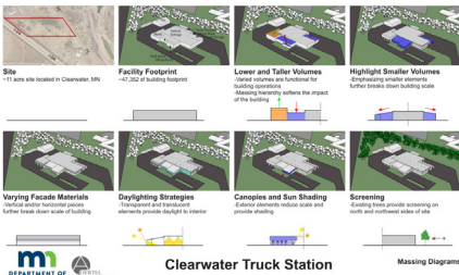
Schematic Design Phase - Massing Diagrams
